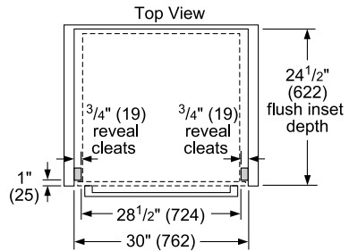
30" Double Wall Oven Flush Installation
