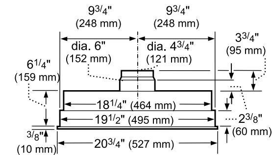
21" HUI31451UC Custom Insert Hood
