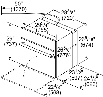
30" Single Wall Oven
