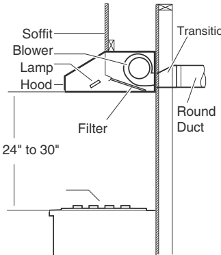
Horizontal discharge
