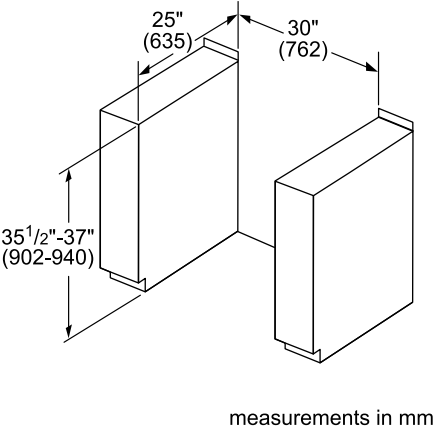
Induction Range Cutout Dimensions
