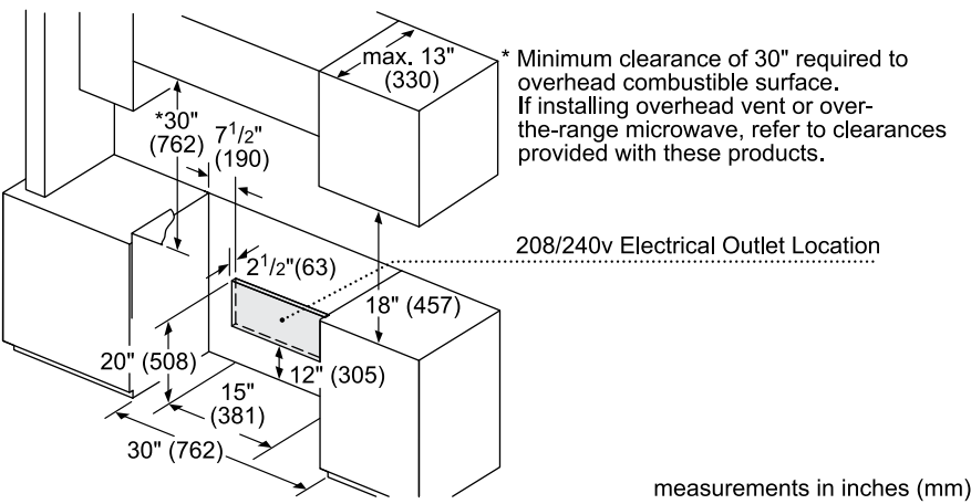
Induction Range Installation
