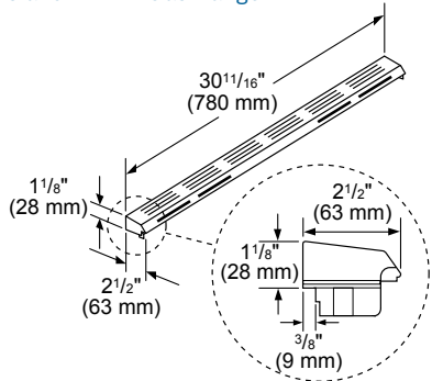
Island Trim – Gas Range
