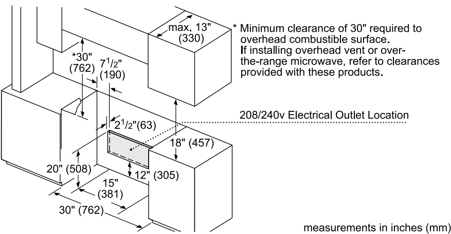
Electric Range Installation
