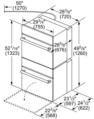
30" Double Wall Oven
