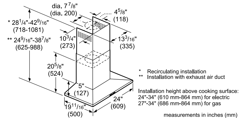
24" HCP34E52UC Pyramid Canopy Chimney Hood
