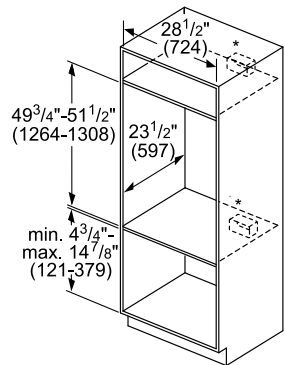
All 30" Double Wall Ovens
