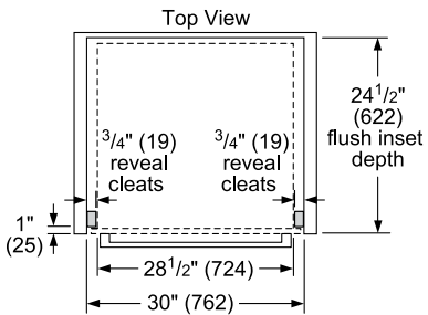
Flush Installation
