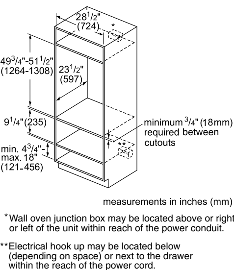
Standard Installation 30" Double Oven over Storage or Warming Drawer
