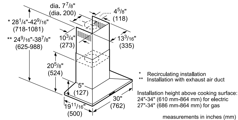
30" HCP30E52UC Pyramid Canopy Chimney Hood
