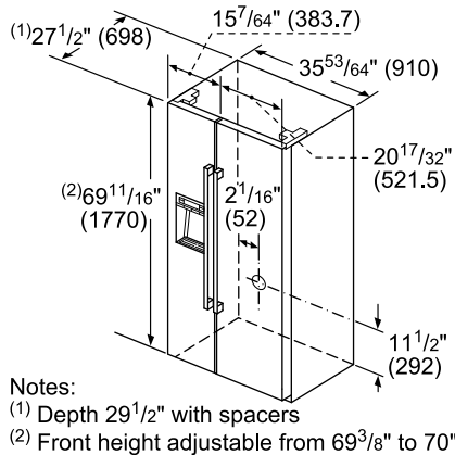
B20CS30SNS Dimensions
