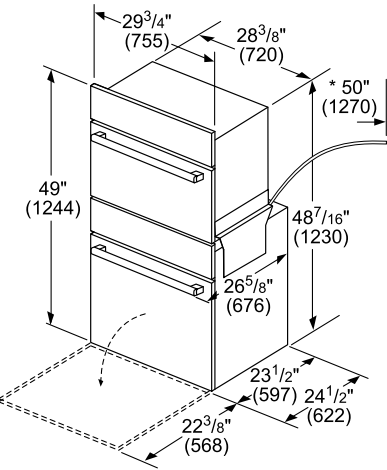
Product Dimensions
