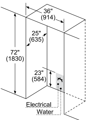
36" Freestanding Installation
