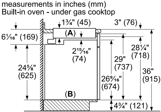
30" & 36" Cooktop Installation Above Wall Oven
