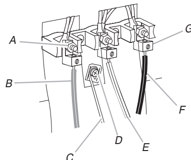
A. 10-32 hex nut B. Line 2 (red) C. Bare (green) ground wire D. Ground-link screw E. Neutral (white) wire F. Line 1 (black) G. Terminal lug
