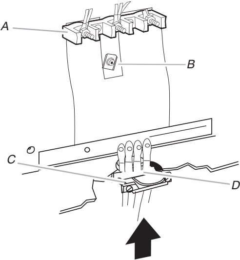
A. Terminal block B. Ground-link screw C. UL listed strain relief D. Power supply cord wire
